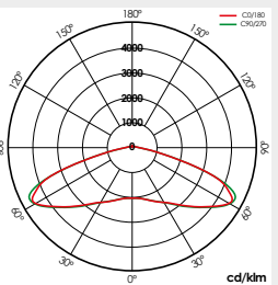
SI50L0M (≤800mA) 64Led
