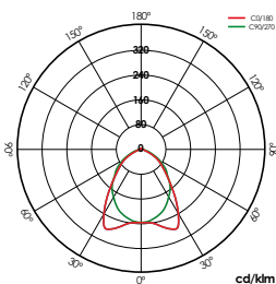
Lynx Led Line
